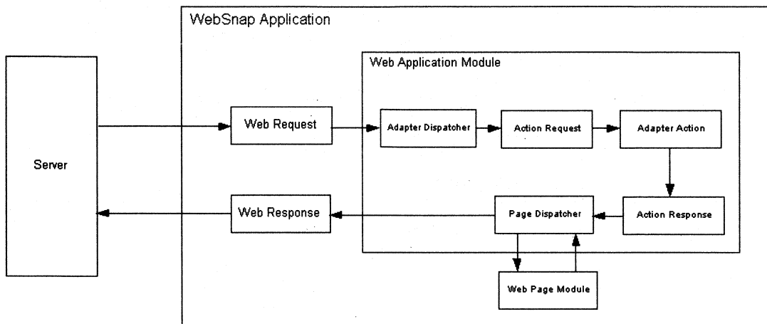
Figure 26.13 Action request and response
