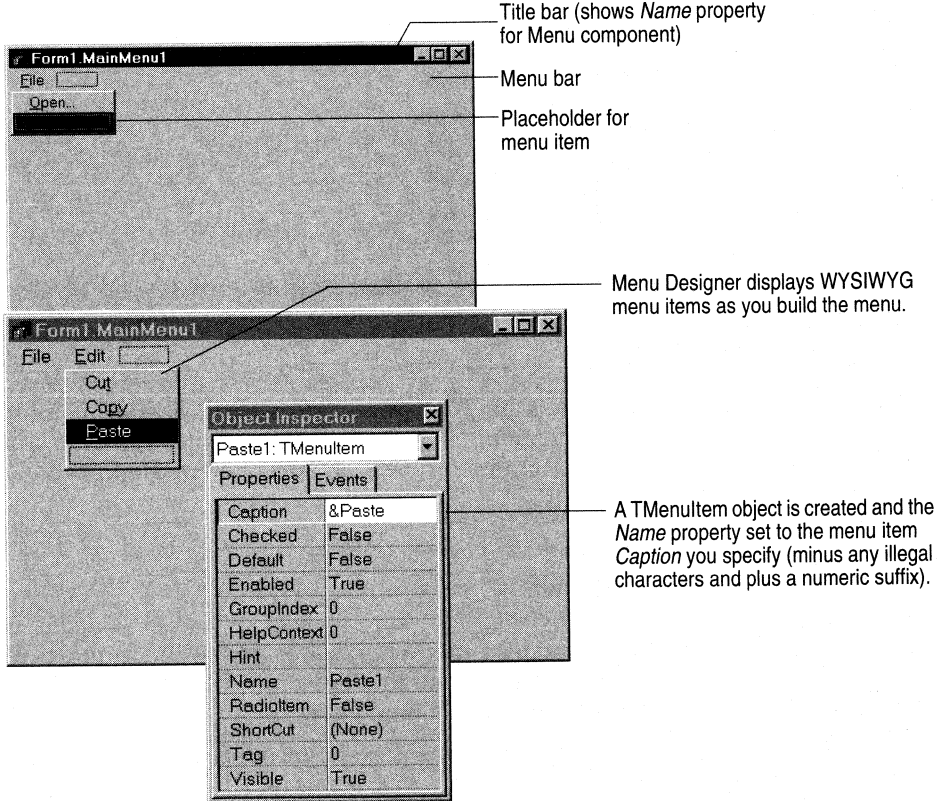
Figure 6.5 Menu Designer for a main menu
