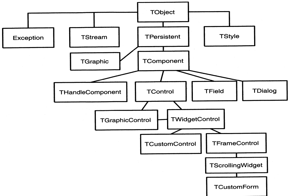
Figure 30.1 CLX class hierarchy
