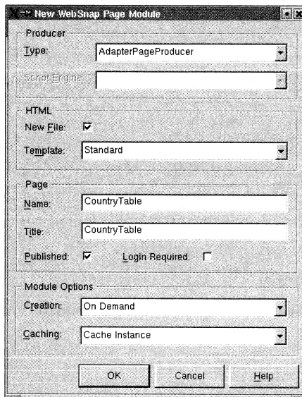
Figure 26.3 New WebSnap Page Module dialog for the CountryTable page
