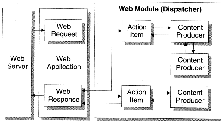
Figure 25.1 Structure of a Server Application
