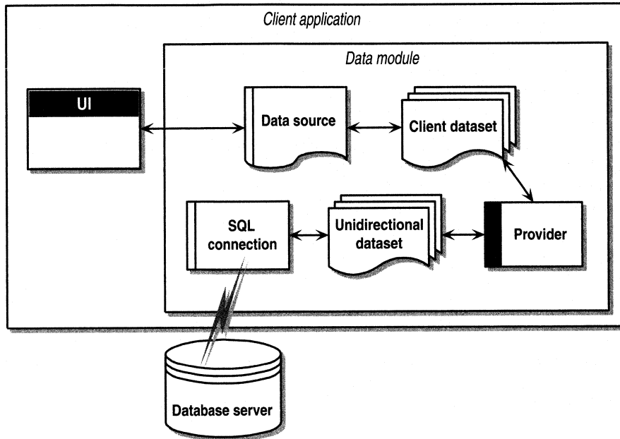
Figure 14.4 Architecture combining a client dataset and a unidirectional dataset
