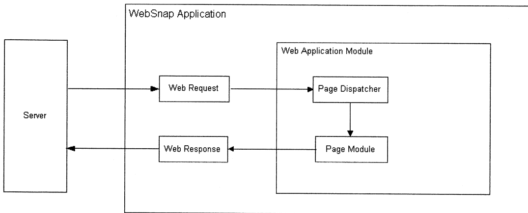
Figure 26.15 Dispatching a page
