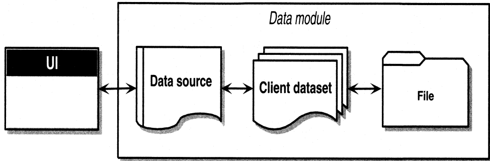
Figure 14.2 Architecture of a file-based database application
