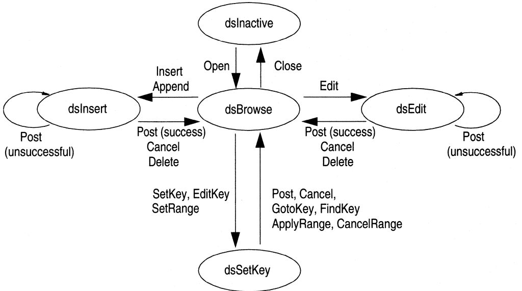
Figure 16.2 Relationship of Browse to other dataset states
