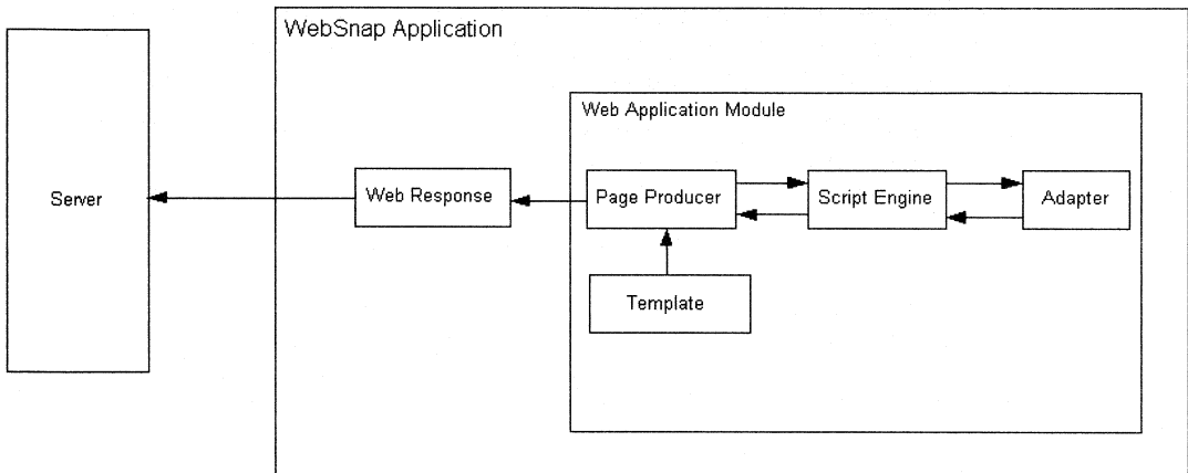
Figure 26.12 Generating content flow
