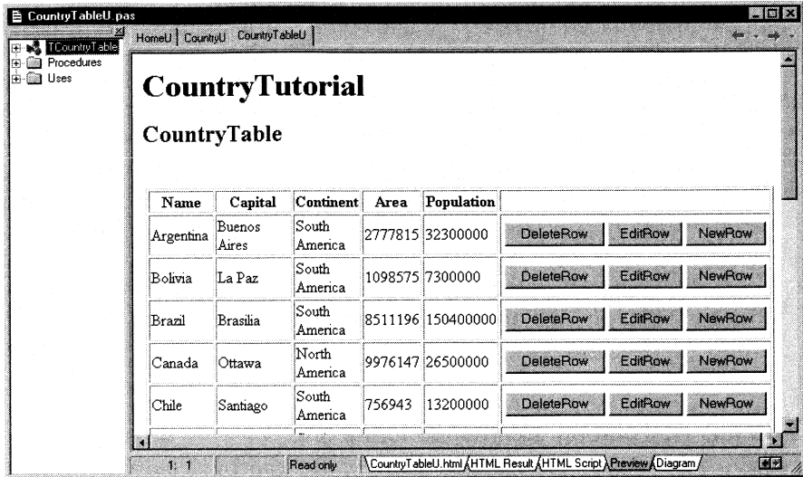
Figure 26.7 CountryTable Preview after adding editing commands
