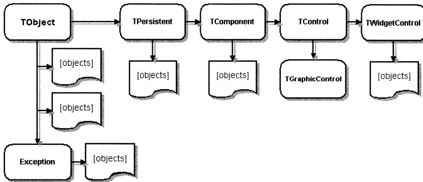
Figure 3.3 A simplified hierarchy diagram
