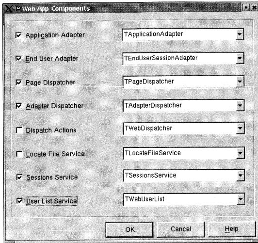
Figure 26.10 Web App Components dialog with options for login support selected
